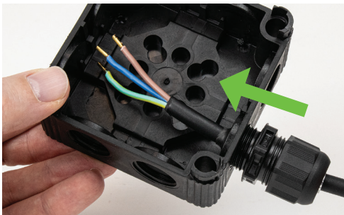
5 Put floodlight wires through gland
