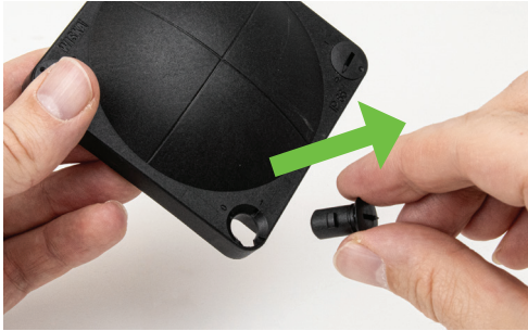
1 Take out locks on WISKA® COMBI® 308
