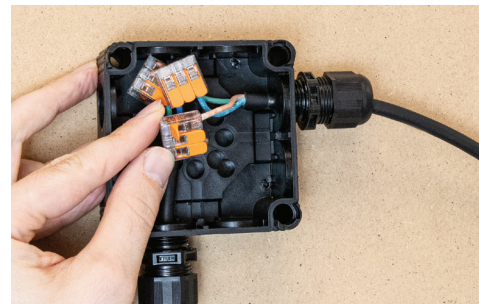
11 Join floodlight cable with mains electricity
