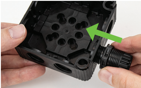
3 Put wire gland into WISKA® COMBI® 308
