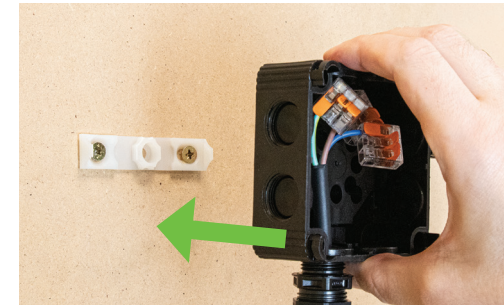
10 Attach WISKA® COMBI® 308 onto mounted wall bracket
